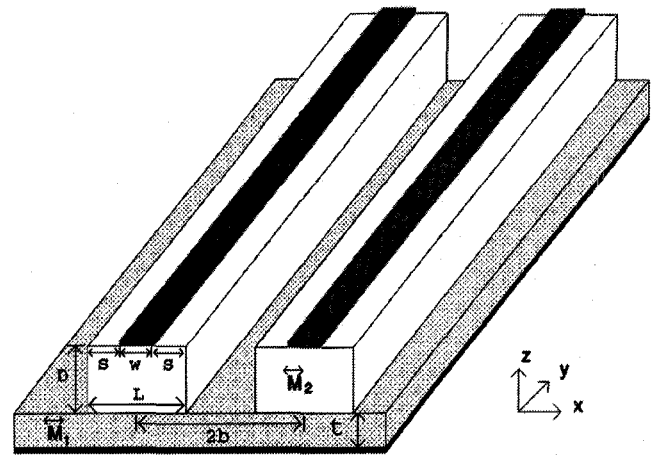
Fig. 1. Complex media microstrip ridge geometry.
