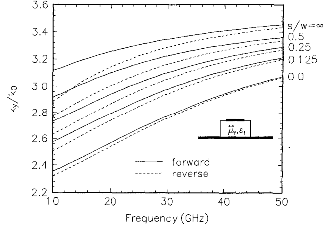
Fig. 2. Dispersion characteristics of a single microstrip ferrite ridge structure for various values of s/w , with D = 0.1016 cm, t = 0 .
